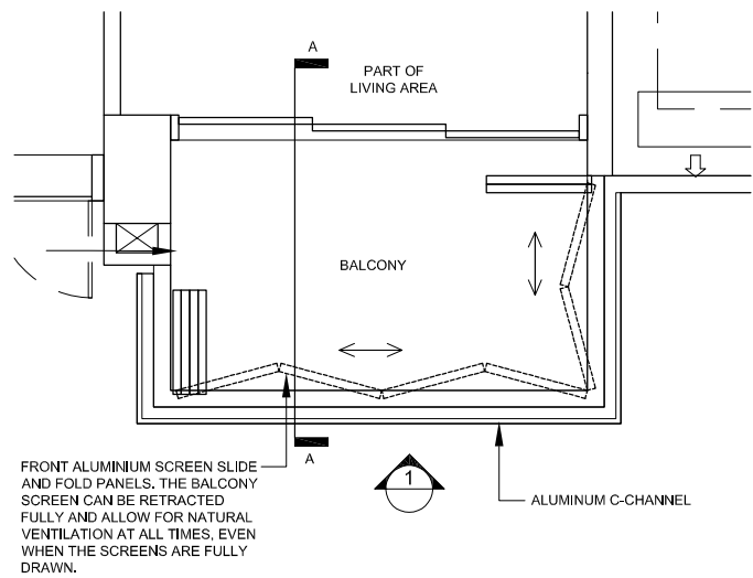
TYPICAL RETRACTABLE BALCONY SCREEN PLAN
